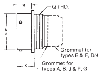
Crimp KPSE01/MS3121
