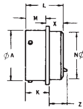
Solder KPT02/MS3112
